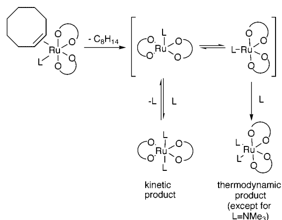
Scheme 2 Suggested pathway for formation of trans - and cis -[Ru(acac) 2 L 2 ] from cis -[Ru(acac) 2 ( \eta^2 -C 8 H 14 )L].
